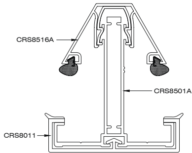
RAFTER ASSEMBLY
