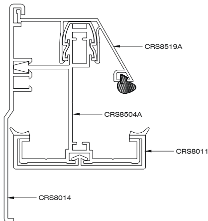
GABLE RAFTER ASSEMBLY
