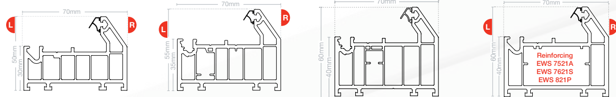
Slim outer frame EWS 7001 Reinforcing EWS 800P Intermediate outer frame EWS 7020 Reinforcing EWS 800P Main frame EWS 7011 Main frame EWS 7021 Reinforcing EWS 7521A EWS 7621S EWS 821P
