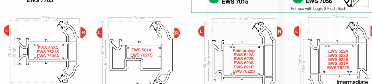
Sash T EWS 7705 EWS 7504A EWS 7604S Sash T EWS 7708 Reinforcing EWS 800P Flush Sash EWS 7015 EWS 7615S Midrail EWS 7056 For use with Logik S Flush Sash
