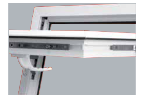
Single hinge and espagnolette location in sashes for ease of fabrication
