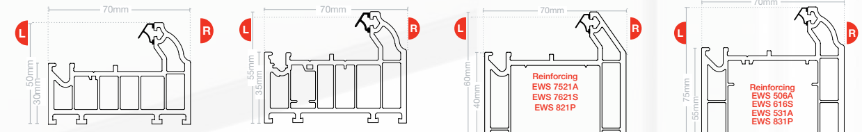
Thermalogik frame EWS 7701 Reinforcing EWS 800P Slim outer frame EWS 7720 Reinforcing EWS 800P Main frame EWS 7721 Reinforcing EWS 7521A EWS 7621S EWS 821P Large main frame EWS 7706 Reinforcing EWS 506A EWS 616S EWS 531A EWS 831P
