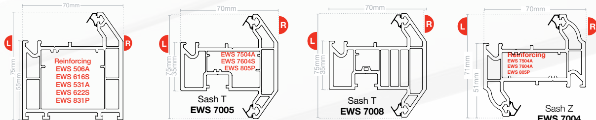
Large main frame EWS 7006 Reinforcing EWS 506A EWS 616S EWS 531A EWS 622S EWS 831P Sash T EWS 7005 EWS 7504A EWS 7604S EWS 805P Sash T EWS 7008 Reinforcing EWS 800P Sash Z EWS 7004 Reinforcing EWS 7504A EWS 7604A EWS 805P
